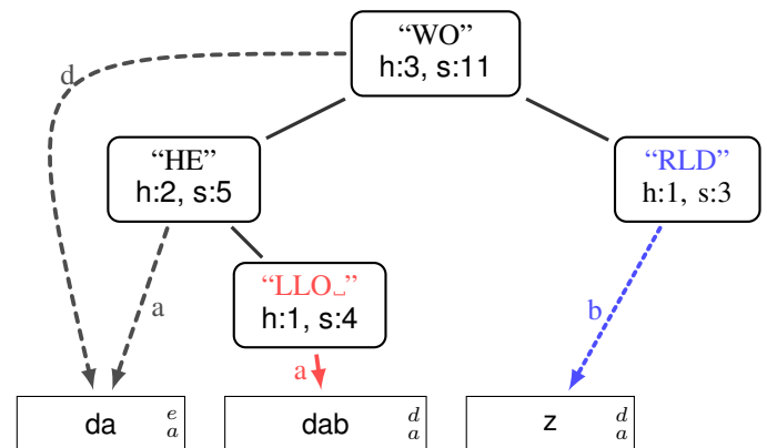
Fig. 3: Tree-based implementation data structures
