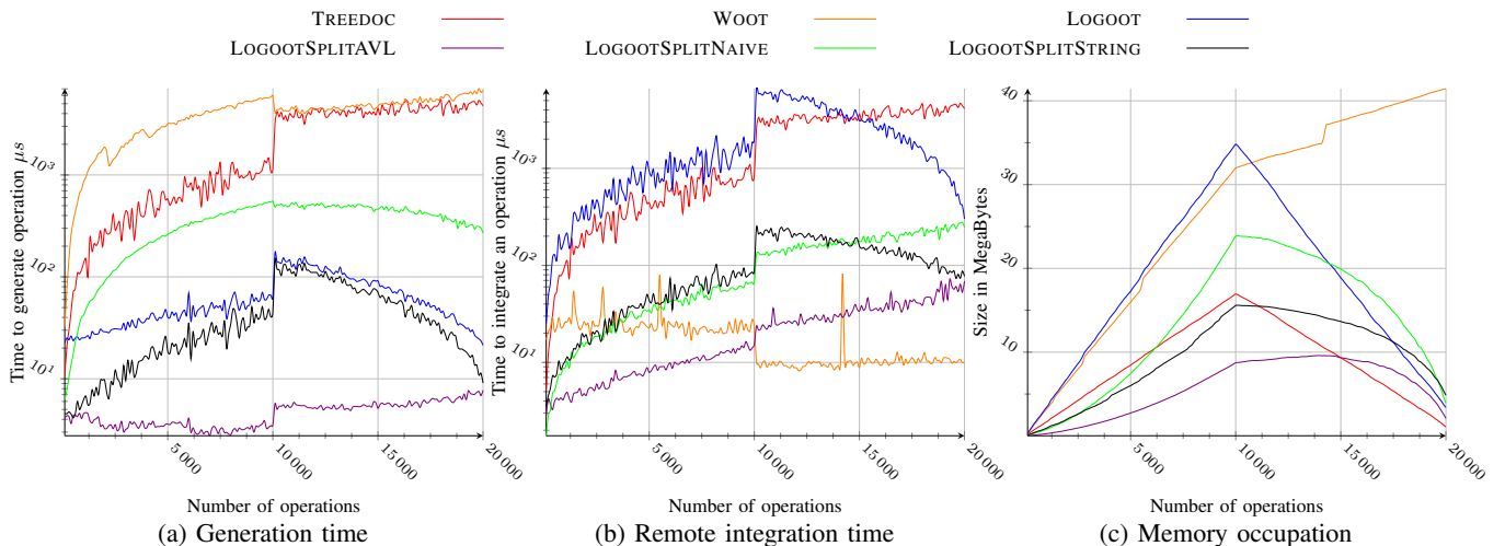
Fig. 5: Experimentation results for trace with right-hand insertions
