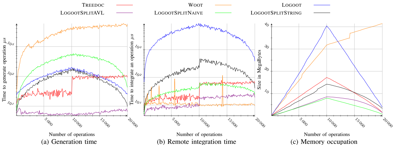
Fig. 4: Experimentation results for random trace
