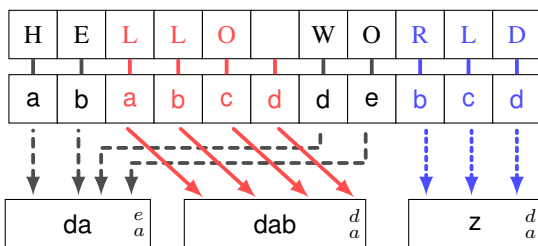
Fig. 2: String-based implementation data structures
